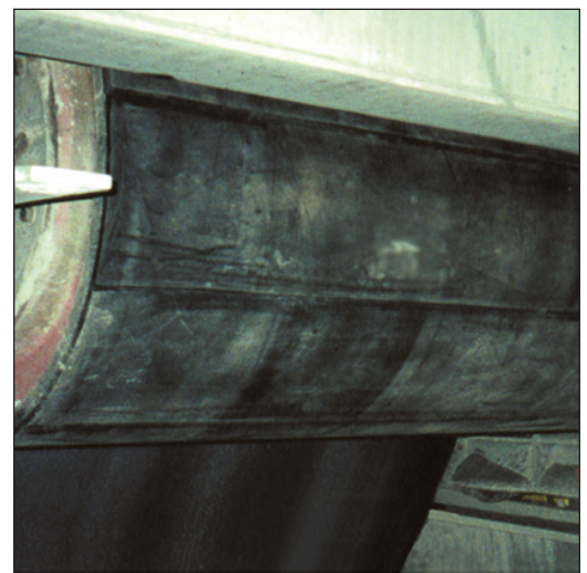
IMTECH ® NDP 60 pulley lagging extends the service life of pulleys in high abrasion applications.
